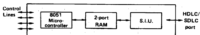
Figure 1. Dual Controller Architecture
