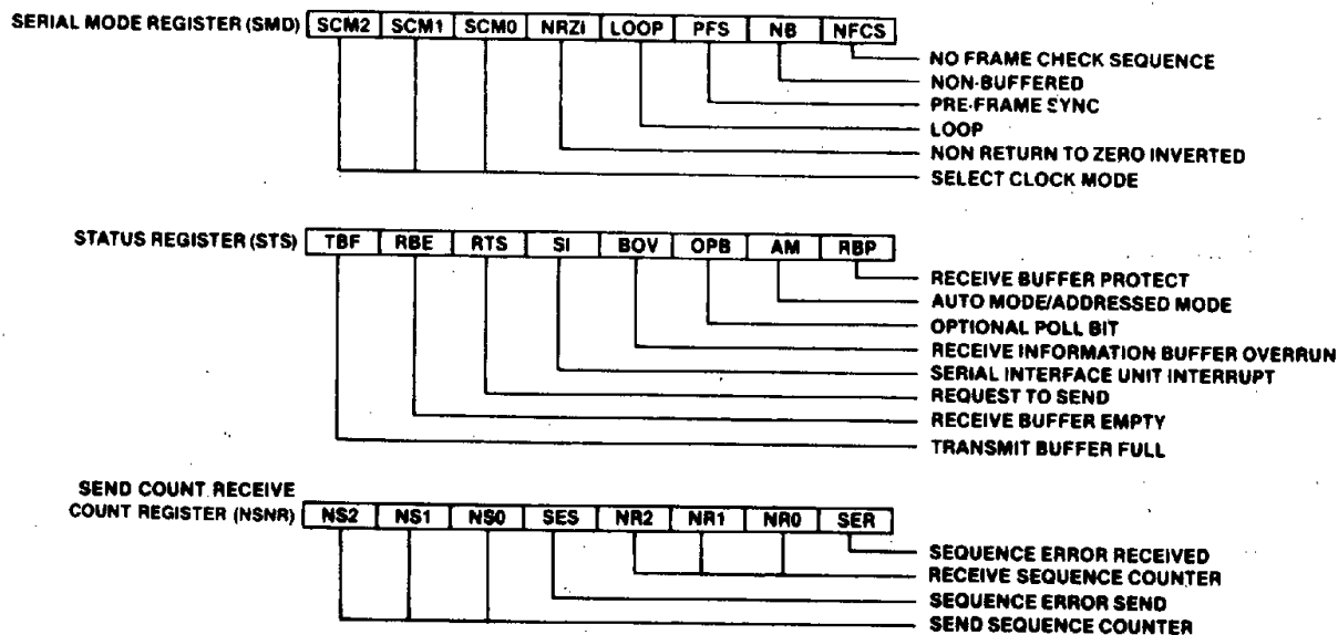
Figure 6. Serial Interface Unit Control Registers
