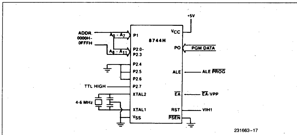
Figure 8. Programming Configuration
