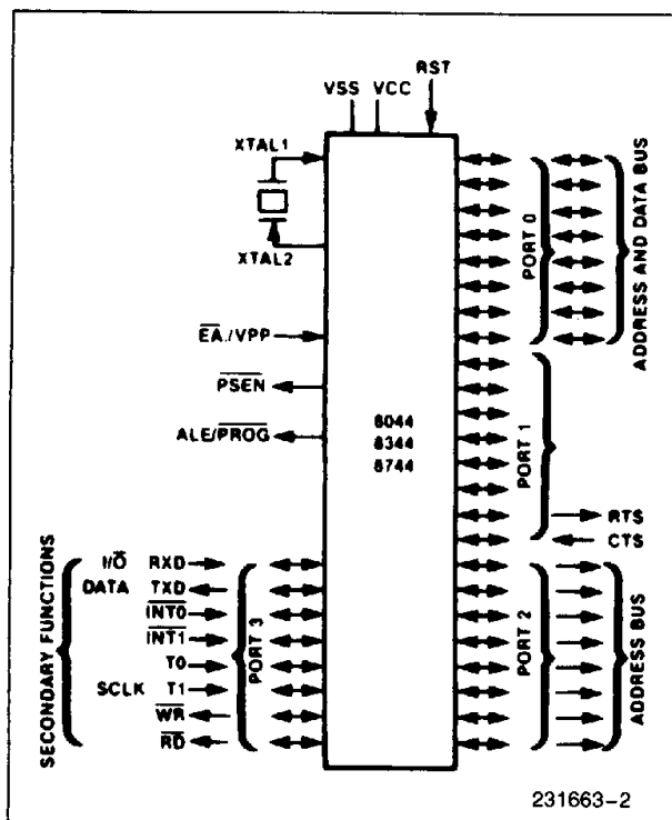
Figure 2. Logic Symbol
